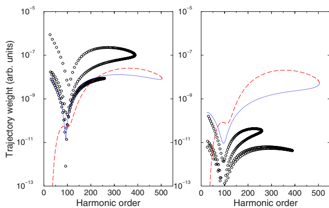
FIG. 7. (Color online) Trajectory weights for 2000 nm wavelength and 2.5 \times 10^{14} W/cm 2 intensity (H 2 only). Left-hand panel: The trajectory weights for the 1L calculation. Right-hand panel: The trajectory weights for the 2L calculation. The red dashed curves are used for the short trajectory and the blue dotted curves are for the long trajectory. The black circles correspond to the longer trajectories. The trajectories shown by the dashed and the dotted lines are used to calculate the ratios depicted by the same curves in Fig. 6.
