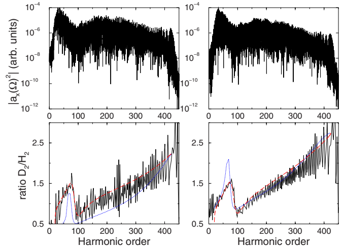
FIG. 4. (Color online) Harmonic generation using 1500 nm laser pulses. Left-hand column, 1L case; right-hand column, 2L case. The upper row shows the harmonic intensities for the H_2 molecule. The lower row shows the harmonic ratio D_2/H_2 (black continuous curve), and the ratio predicted if one takes into account the short trajectory only (red dashed curve) or the long trajectory only (blue dotted curve).
