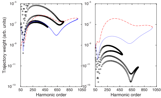
FIG. 9. (Color online) Trajectory weights for 2000 nm wavelength and 5 \times 10^{14} W/cm 2 intensity. Left-hand panel: The trajectory weights for the 1L calculation. Right-hand panel: The trajectory weights for the 2L calculation. The red dashed curves are used for the short trajectory and the blue dotted curves are for the long trajectory. The black circles correspond to the longer trajectories. The trajectories shown by the dashed and the dotted lines are used to calculate the ratios depicted by the same curves in Fig. 8.
