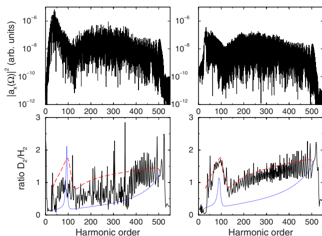
FIG. 6. (Color online) Harmonic generation using 2000 nm laser pulse with 2.5 \times 10^{14} W/cm 2 intensity. Left-hand column, 1L case; right-hand column, 2L case. The upper row shows the harmonic intensities for the H 2 molecule. The lower row shows the harmonic ratio D_2/H_2 (black continuous curve), and the ratio predicted if one takes into account the short trajectory only (red dashed curve) or the long trajectory only (blue dotted curve).
