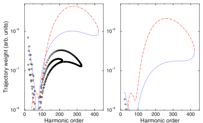
FIG. 5. (Color online) Trajectory weights for 1500 nm wavelength ( H_2 only). Left-hand panel: The trajectory weights for the 1L calculation. Right-hand panel: The trajectory weights for the 2L calculation. The red dashed curves are used for the short trajectory and the blue dotted curves are used for the long trajectory. The black circles correspond to the longer trajectories. The trajectories shown by the dashed and the dotted lines are used to calculate the ratios depicted by the same curves in Fig. 4.
