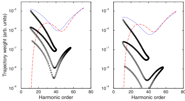
FIG. 3. (Color online) Trajectory weights for 800 nm laser pulses ( H_2 only). Left-hand panel: The trajectory weights for the 1L calculation. Right-hand panel: The trajectory weights for the 2L calculation. The red dashed curves are used for the short trajectory and the blue dotted curves are for the long trajectory. The black circles correspond to the longer trajectories. The trajectories shown by the dashed and the dotted lines are used to calculate the ratios depicted by the same curves in Fig. 2.
