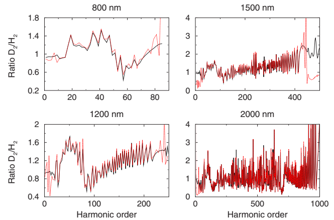
FIG. 11. (Color online) Comparison between the full calculation (black curves) based on Eq. (4) and by using the saddle-point approximation (red dotted curves). The calculations are for the 1L case.
