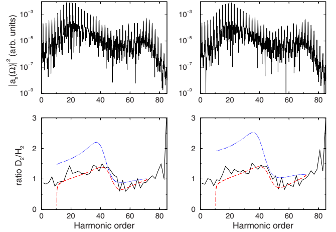
FIG. 2. (Color online) Harmonic generation using 800 nm laser pulses. Left-hand column, 1L case; right-hand column, 2L case. The upper row shows the harmonic intensities for the H_2 molecule. The lower row shows the harmonic ratio D_2/H_2 (black continuous curve), and the ratio predicted if one takes into account the short trajectory only (red dashed curve) or the long trajectory only (blue dotted curve).
