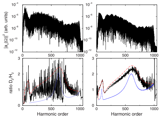
FIG. 8. (Color online) Harmonic generation using 2000 nm laser pulses with 5 \times 10^{14} W/cm 2 intensity. Left-hand column, 1L case; right-hand column, 2L case. The upper row shows the harmonic intensities for the H 2 molecule. The lower row shows the harmonic ratio D_2/H_2 (black continuous curve), and the ratio predicted if one takes into account the short trajectory only (red dashed curve) or the long trajectory only (blue dotted curve).
